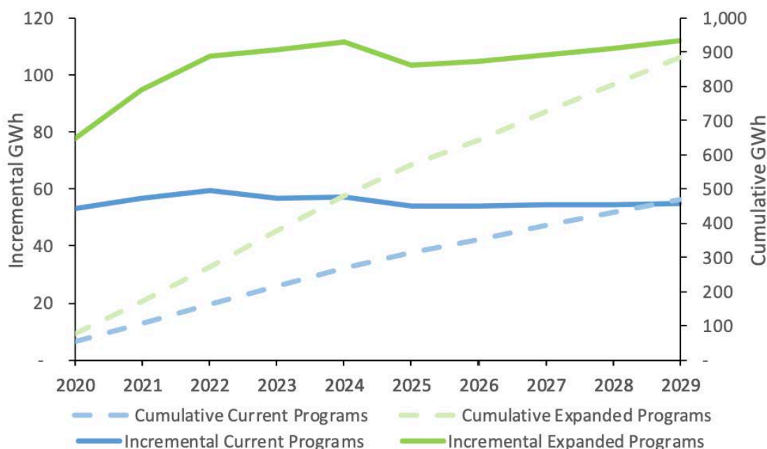
Figure 3. Dominion Energy SC Incremental and Cumulative Portfolio Energy Savings
